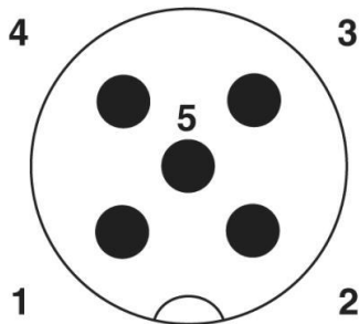
5-poles M12 A-coded male connector
